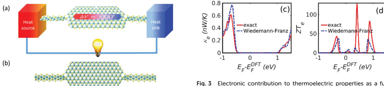
Fig. 1 (a) Schematic of Mo 6 S 6 nanowire–MoS 2 –Mo 6 S 6 nanowire junction. (b) The Mo 6 S 6 –MoS 2 –Mo 6 S 6 junction used in the simulation: yellow atoms represent sulphur and green represents molybdenum.
