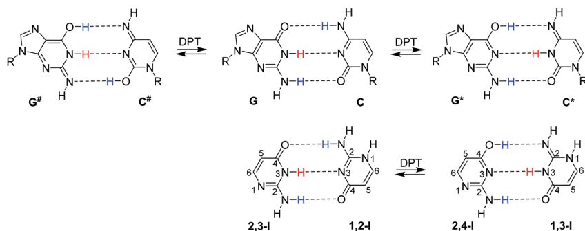
Fig. 1 Top: canonical G–C base pair and two G–C base pairs resulting after DPT: G * –C * and G # –C # . Bottom: dimer of isocytosine found in its crystalline phase, consisting of 1,2-I and 2,3-I tautomers, and the isocytosine dimer after DPT.
