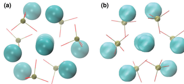
Fig. 1 Projection on the xy plane of (a) Posner's cluster in hydroxyapatite, C3 symmetry; (b) Posner's cluster in water, simulated with the force field of Ainsworth et al. 18 Colour key Ca: light blue, P: green, O: red.
