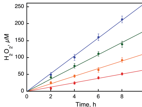
Fig. 4 Time courses of the photocatalytic production of \text{H}_2\text{O}_2 from \text{H}_2\text{O} and \text{O}_2 with [\text{Ru}^{\text{II}}(\text{Me}_2\text{phen})_3]^{2+} ( 0.10 \text{mM} ) in the presence of a catalytic amount of 1 [ 0.50 \text{mM} (red), 1.0 \text{mM} (orange), 1.5 \text{mM} (green), and 2.0 \text{mM} (blue)] in an air-saturated solvent mixture of MeCN and \text{H}_2\text{O} ( v/v = 23 : 2 ) containing \text{Sc}(\text{NO}_3)_3 ( 100 \text{mM} ) under photoirradiation (white light) at 298 \text{K} .
