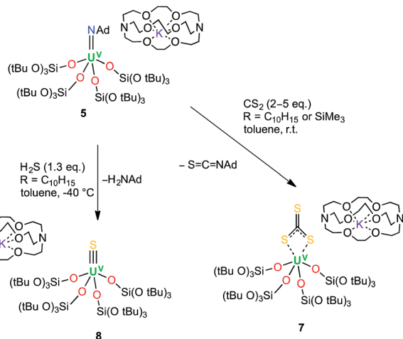
Scheme 3 Syntheses of the terminal U V trithiocarbonate complex, [K(2.2.2-cryptand)][U(CS 3 ){OSi(O t Bu) 3 ] 4 ] ( 7 ), and the terminal U V sulfide complex, [K(2.2.2-cryptand)][U(S{OSi(O t Bu) 3 )] 4 ] ( 8 ).
