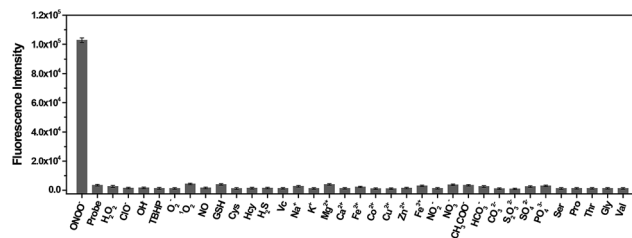
Fig. 1 Fluorescence response of TP-KA (1.0 \mu M) with various bioanalytes, including ONOO - (10.0 \mu M), H 2 O 2 (200 \mu M), other ROS and RNS (10.0 \mu M), GSH and Cys (5.0 mM), and other interfering substances (100 mM). The data were recorded after the incubation of TP-KA with various bioanalytes for 10 min at 37 ^{\circ} C in PBS buffer (50 mM, 7.4) with 1% DMSO. The values are the mean \pm s.d. for n = 3 . \lambda_{\text{ex}}/\lambda_{\text{em}} = 430/560 nm.
