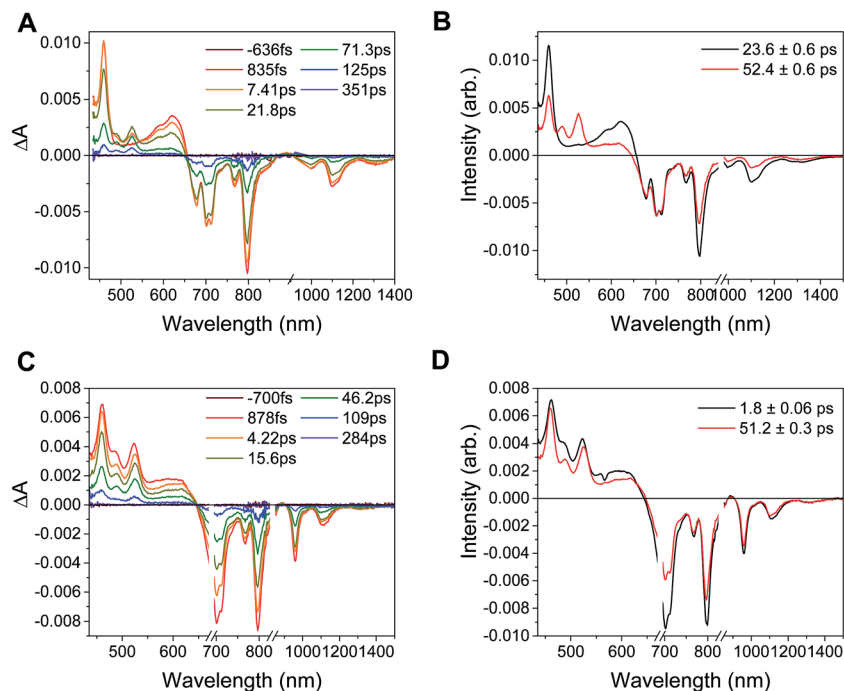
Fig. 6 Top: (A) Transient absorption spectra and (B) decay-associated spectra for \text{PDI}^{1-} -Phbpy-Re-Py ( \lambda_{\text{ex}} = 950 nm). (C) Transient absorption spectra and (D) decay-associated spectra of those spectra for \text{PDI}^{1-} -Phbpy-Re-Py ( \lambda_{\text{ex}} = 680 nm).
