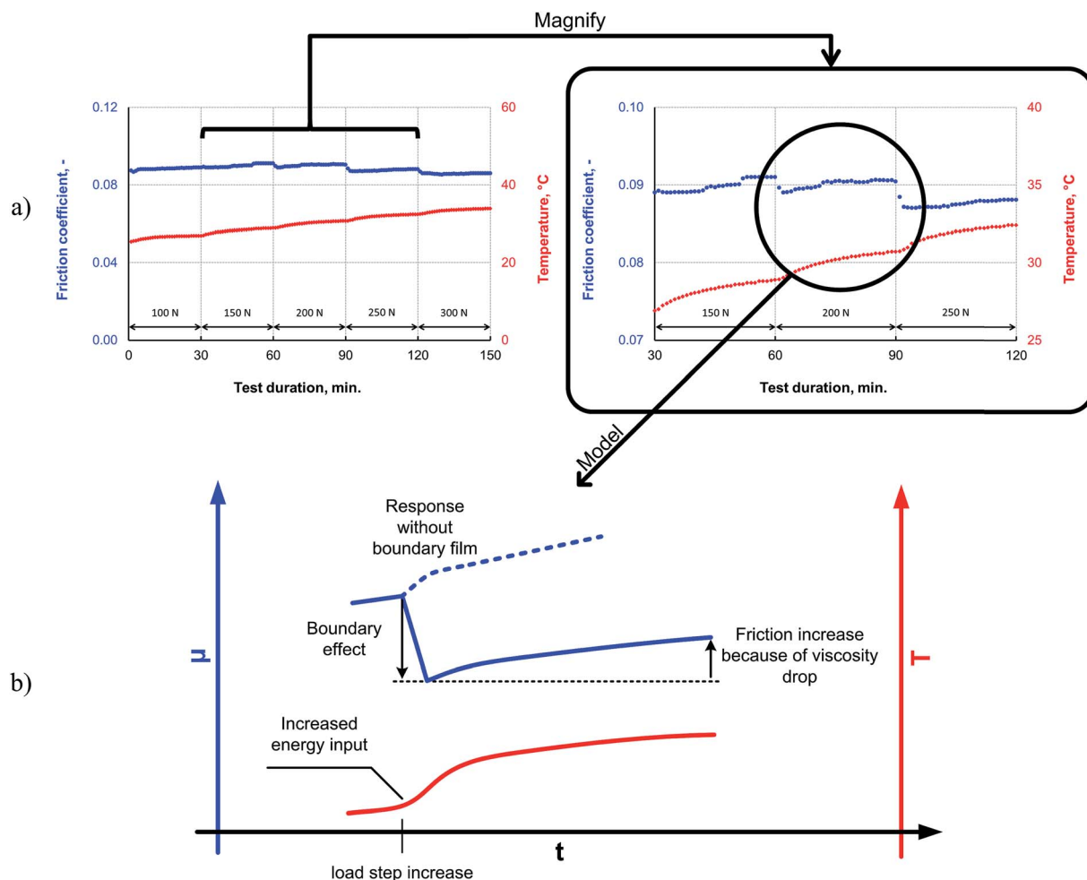
Fig. 9 P-SiSO[4-16][1-2] evaluated by increasing the applied load in a stepwise manner during the reciprocating tribotest performed under the conditions V\{100-300\text{ N}/25\text{ }^\circ\text{C}/150\text{ min}\} ; data shown in (a). The friction response to the stepwise increase in the load indicates the formation of a friction-reducing boundary film, as shown schematically in (b).
