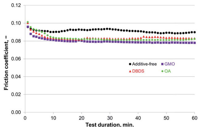
Fig. 10 Compatibility of additives for use with P-SiSO[4-16][1-2] evaluated by the reciprocating tribotests performed under conditions of C\{100\text{ N}/75\text{ }^\circ\text{C}/60\text{ min}\} .
