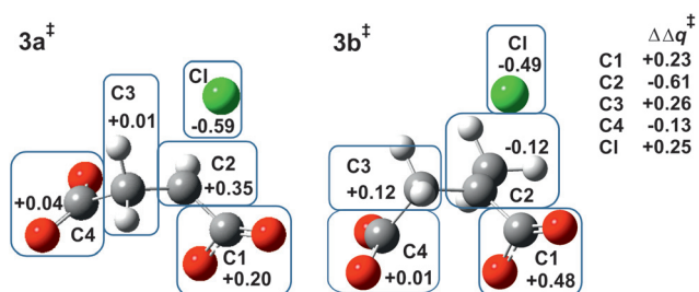
Fig. 2 Changes in MP2-PCM/6-311+G(d,p) ESP atomic charges ( \Delta q^{\ddagger}/|e| ) summed over the atoms within each boxed group, from chlorosuccinate 1a or 1b to TS 3a ‡ or 3b ‡ , respectively, together with differential changes ( \Delta\Delta q^{\ddagger} ).
