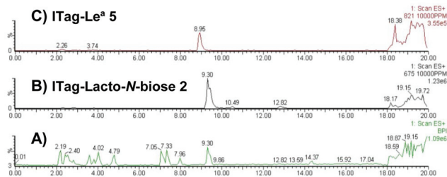
Scheme 4 Incubation of ITagged 2 with GDP-Fuc in HBM to obtain ITag-Lewis a 5 ( M^+ 821) and LC-MS traces of: (A) total ion count of HBM reaction mixture; (B) extracted LC-MS trace for 2 ( M^+ 675) and (C) extracted LC-MS trace for 5 ( M^+ 821).
