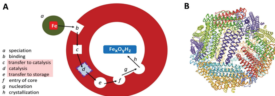
Fig. 1 (A) Schematic outline of phases involved in the uptake, oxidation, and storage of \text{Fe(II)} by ferritin; (B) the conserved nanocage structure of 24-meric ferritin (taken from ref. 2).
