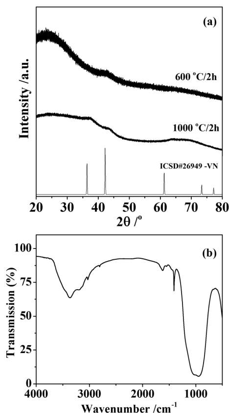
Fig. 2 Powder XRD pattern from the silicon–vanadium nitride nanocomposites (a) and infrared spectrum of the sample synthesised at 1000 ^\circ\text{C} (b). The XRD patterns are compared with crystalline VN from ICSD file 26949. 32
