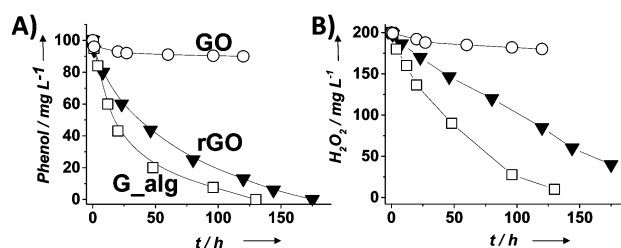
Fig. 3 Temporal profiles of phenol degradation (A) and consumed H 2 O 2 (B) using G-based catalysts. Legend: G (□), rGO (▼) and GO (○). Reaction conditions: catalyst (200 mg L -1 ), phenol (100 mg L -1 , 1.06 mM), H 2 O 2 (200 mg L -1 , 5.88 mM), pH 3, room temperature. Reproduced from ref. 58 with permission from Wiley, copyright 2017.
