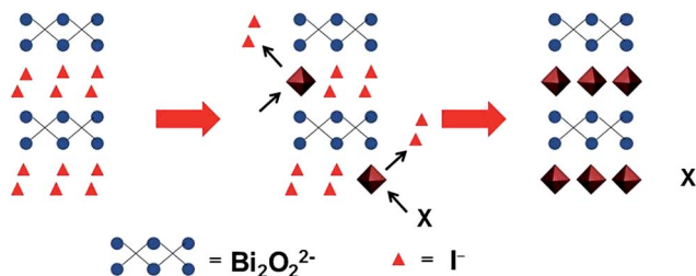
Scheme 1 Schematic illustration of the hydrothermal anion exchange: from BiOI to Bi-based binary metal oxide. X = \text{WO}_4^{2-} , \text{VO}_3^- or \text{MoO}_4^{2-} .
