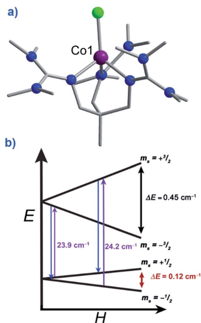
Fig. 21 (a) Molecular structure of [(3G)CoCl](CF 3 SO 3 ) (58). Colour code: purple (Co), bright green (Cl), blue (N), grey (C). Hydrogen atoms omitted for clarity. (b) Zeeman splitting diagram for 58, where the red arrows indicated the direct relaxation process, the purple arrows correspond to the excitation energies related to the Orbach processes, and the blue arrows correspond to the relaxation via the Orbach process. All values presented were determined for S = 3/2 , g , D , and E as determined by EPR spectroscopy. Reprinted with permission from ref. 65. Copyright (2012) Royal Society of Chemistry.
