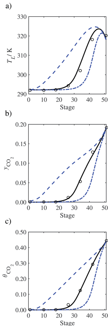
Fig. 21 Sensitivity analysis of the liquid viscosity on the profiles predicted with our model compared with the experimental pilot-plant data of Run T22 of Tontiwachwuthikul et al. 13 nominal value (continuous curve), viscosity doubled (dashed curve), and viscosity halved (dot-dashed curve). (a) Temperature profile for the liquid phase, (b) gas-phase CO 2 concentration profile, and (c) liquid-phase CO 2 loading.
