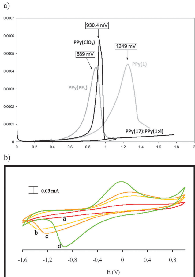
Fig. 7 (a) LSV studies of PPy(PF 6 ), PPy(CIO 4 ), PPy(1) and copolymer PPy(17):PPy (1:4). LSV consists of the measurement of the current associated with overoxidation during a single scan (0 to 1.5 V vs. Ag/AgCl) at low scan rate (0.5 mV s -1 ) in a 0.5 M KCl solution. (b) Gradual self-repairing of copolymer PPy(17):PPy shown by ion exchange tests in NaCl 0.1 M: (a) immediately after destabilizing the PPy(17):PPy by applying 1300 mV, (b) after 30 minutes in the same electrolytic solution, (c) after 1 h and (d) after 18 h.
