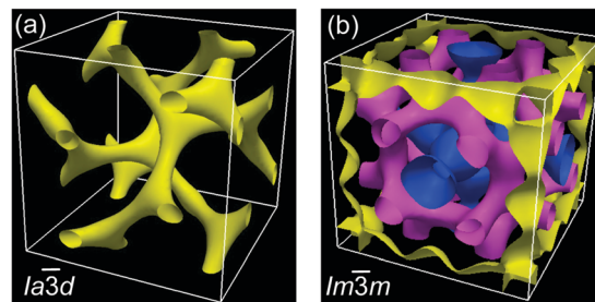
Fig. 4 Reconstructed EDMs: (a) of a unit cell of the Cub/ Ia\bar{3}d phase of AB8 only showing the high density regions and (b) of the Im\bar{3}m approximate of the Cub/ I432 phase of AB14 showing the three distinct iso-surfaces with different colour.
