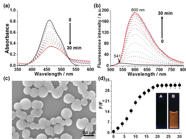
Fig. 1 Absorption (a) and fluorescence emission (b) spectra of probe 1-SO 3 − (20 \mu\text{M} ) upon incubation with spermine (20 \mu\text{M} ) for different time periods in HEPES buffer (10 mM, pH = 7.4) at 25 °C. The spectra were obtained every 2 min (0–30 min). The black solid line and red solid line indicate spectra of probe 1-SO 3 − before and 30 min after addition of spermine, respectively. Excited at 470 nm. (c) SEM image of the dried aggregates, formed from a solution of the probe 1-SO 3 − (20 \mu\text{M} ) upon 20 min incubation with spermine (20 \mu\text{M} ) in HEPES buffer (10 mM, pH = 7.4) at 25 °C. (d) Relative fluorescence intensity ( F/F_0 ) of probe 1-SO 3 − (20 \mu\text{M} ) as a function of incubation time with spermine (20 \mu\text{M} ). F and F_0 correspond to the fluorescence intensity of 1-SO 3 − in the presence and absence of spermine, respectively. The values were obtained at \lambda_{\text{em}} = 600 \text{ nm} . Inset shows photographs of probe 1-SO 3 − in the absence (A) and presence (B) of spermine after incubation for 30 min under irradiation with UV light at \lambda = 365 \text{ nm} . [ 1-SO 3 − ] = [spermine] = 20 \mu\text{M} .
