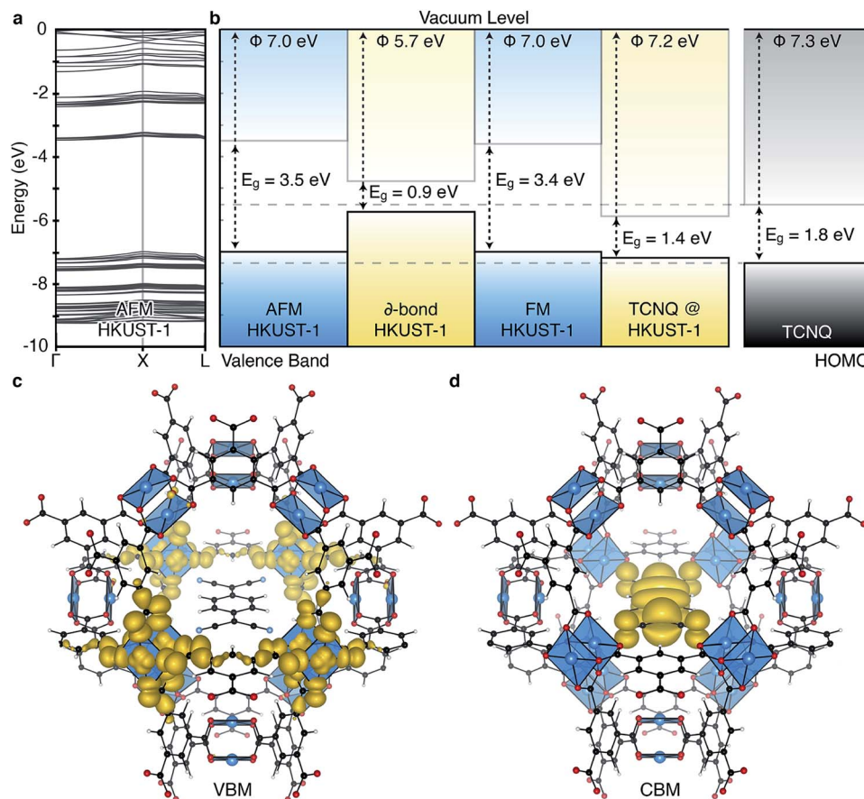
Fig. 4 The electronic band structure of HKUST-1 in the antiferromagnetic (AFM) configuration, a , shows typical behaviour of a metal–organic framework: bands with low dispersion in reciprocal space indicating highly localised states. The three spin states per Cu···Cu paddlewheel considered result in three distinct ionisation potentials (workfunctions), shown relative to the vacuum level in (b) . Inclusion of the TCNQ electron acceptor in the pores of HKUST-1 provides an electron acceptor and transport medium. Solid-state calculations of the TCNQ/HKUST-1 interface show the upper valence band of the framework is not affected by the inclusion of TCNQ, (c) , however the molecular LUMO occupies a mid-gap state, (d) . All calculations are based on a density functional theory with a hybrid exchange–correlation functional (HSE06).
