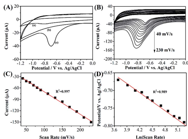
Fig. 3 (A) CVs of bare (a) GCE, (b) and (c) RGO-Au/GCE in 0.1 M PBS (pH 7.0) with and without 10 \mu\text{M} phoxim. Scan rate: 50 \text{mV s}^{-1} . (B) CVs of RGO-Au/GCE in 10 \mu\text{M} phoxim at different scan rates (40, 50, 60, 70, 80, 90, 110, 130, 150, 170, 190, 210 and 230 \text{mV s}^{-1} ). (C) The plot for the dependence of peak current on the scan rate. (D) The relationship between E_{\text{pa}} and \ln v .
