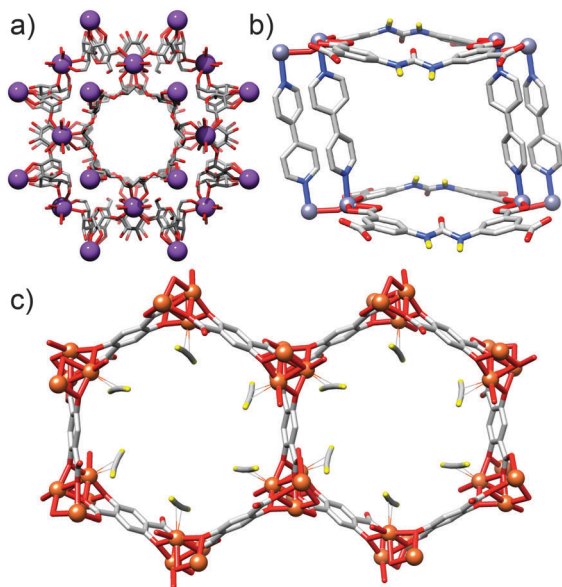
Fig. 1 Sections of the solid-state structures of (a) CD-MOF-2, whose surfeit of pendant hydroxyl units facilitates transient chemisorption of \text{CO}_2 , (b) NU-601, a urea functionalised MOF which acts as a heterogeneous organocatalyst, and (c) iron dioxidoterephthalate, binding acetylene through interactions with coordinatively unsaturated \text{Fe}^{2+} cations. Redrawn from CSD depositions LAJLEP, HAPHUD and SARGID, in turn.
