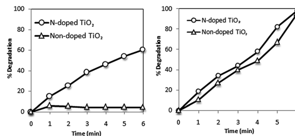
Fig. 4 Photocatalytic degradation of direct black 38 as a function of time under visible light (left) and sunlight (right). Experimental conditions: C_0 = 0.055 \text{ g L}^{-1} , C_{\text{catalyst}} = 1.0 \text{ g L}^{-1} , \text{pH} = 2.5 , T = 25^\circ \text{C} . 153
