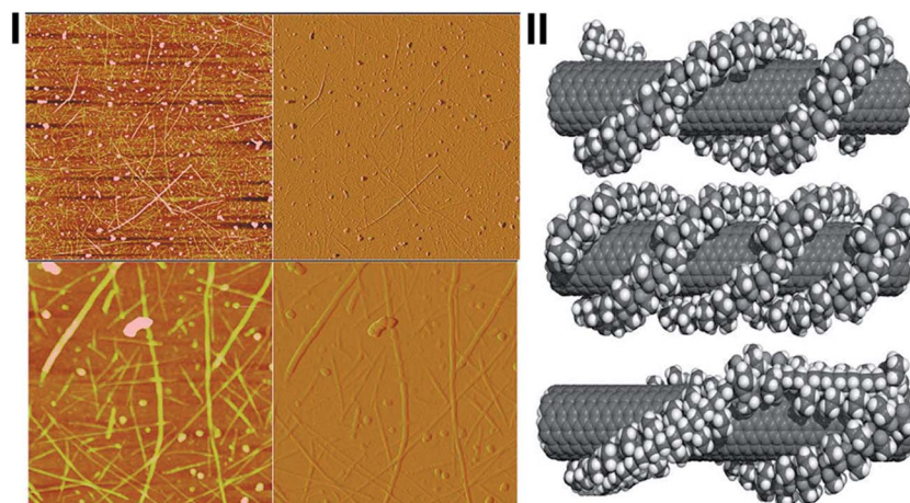
Fig. 6 (I) Tapping-mode AFM images of PVP-SWNTs on a functionalized substrate. 5 \mu\text{m} height (top left) and amplitude image (top right). 1 \mu\text{m} expanded height image (bottom left) and amplitude image (bottom right). (II) Some possible wrapping arrangements of PVP on an 8, 8 SWNT. A double helix (top) and a triple helix (middle). Backbone bond rotations can induce switch-backs, allowing multiple parallel wrapping strands to come from the same polymer chain (bottom) (after ref. 112 reproduced with permission).
