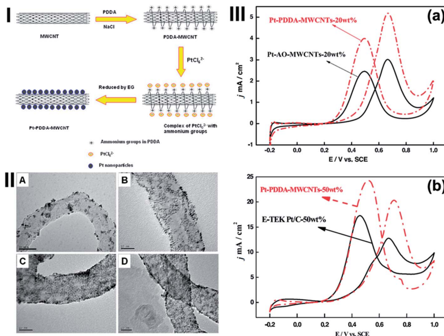
Fig. 7 (I) Scheme of PDDA functionalization of MWCNTs and the in situ synthesis of Pt nanoparticles on PDDA-functionalized MWCNTs. (II) TEM images of (a) Pt-AO-MWCNTs-20 wt%, (b) Pt-PDDA-MWCNTs-20 wt%, (c) Pt-PDDA-MWCNTs-40 wt%, (d) Pt-PDDA-MWCNTs-60 wt%. (III) (a) CVs of Pt catalysts supported on PDDA-MWCNTs and AO-MWCNTs in nitrogen saturated 0.5 M H 2 SO 4 + 1.0 M CH 3 OH. (b) CVs of Pt-PDDA-MWCNTs-50 wt% and E-TEK Pt/C (50 wt%) in nitrogen purged 0.5 M H 2 SO 4 + 1.0 M CH 3 OH. The Pt loading was 0.05 mg cm -2 (after ref. 67 reproduced with permission).
