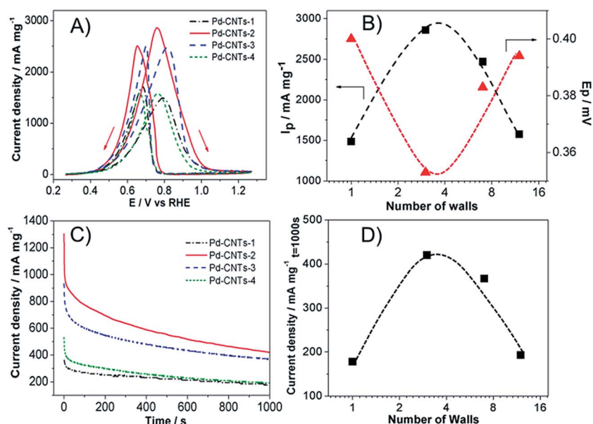
Fig. 14 (A) Cyclic voltammetry curves of Pd-CNTs catalysts for ethanol oxidation reaction (EOR), measured in a 1.0 M ethanol + 1.0 M KOH solution at scan rate 50 \text{ mV s}^{-1} , (B) plots of peak current density and onset potential of EOR against wall numbers of CNTs, (C) chronoamperometry curves of Pd-CNTs catalysts for EOR, measured at 0.67 \text{ V} in a 1.0 M ethanol + 1.0 M KOH solution, (D) plots of current density measured at t = 1000 \text{ s} for EOR. Pd loading was 0.05 \text{ mg cm}^{-2} (after ref. 161 reproduced with permission).
