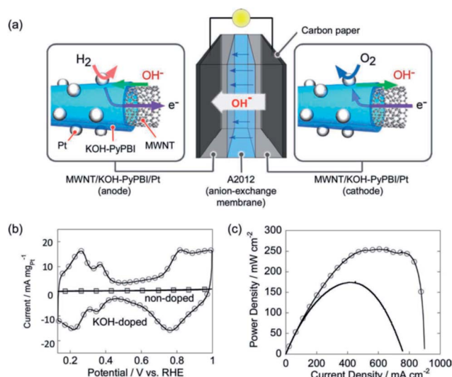
Fig. 9 (a) Schematic illustration of the KOH doped PyBBI cell. Mass transfer in the cell is also shown. (b) In situ CVs of cathode in the KOH-doped MEA (circles) and non-doped MEA (squares) at a scan rate of 50 mV s -1 . (c) Power density curves of the KOH-doped MEA (circles) and standard MEA (black line) (after ref. 127 reproduced with permission).
