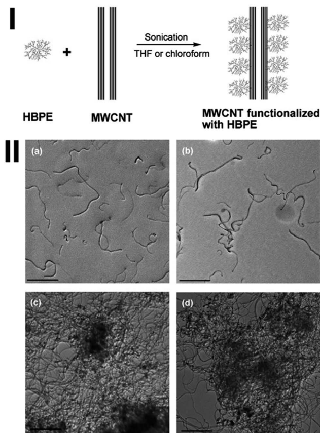
Fig. 5 (I) Schematic noncovalent nonspecific functionalization and solubilization of MWCNTs with HBPE. (II) TEM images of (a) MWCNTs solubilized with HBPE in chloroform; (b) MWCNTs solubilized with HBPE in THF; (c) MWCNTs dispersed with HBPE in toluene; (d) pristine MWCNTs dispersed in heptane. In (a)–(c), the same HBPE/MWCNT mass ratio of 0.4 was used. Scale bar: 500 nm (after ref. 106 reproduced with permission).
