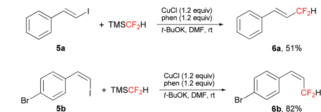
Scheme 2 Copper-mediated difluoromethylation of β-styryl iodides.
