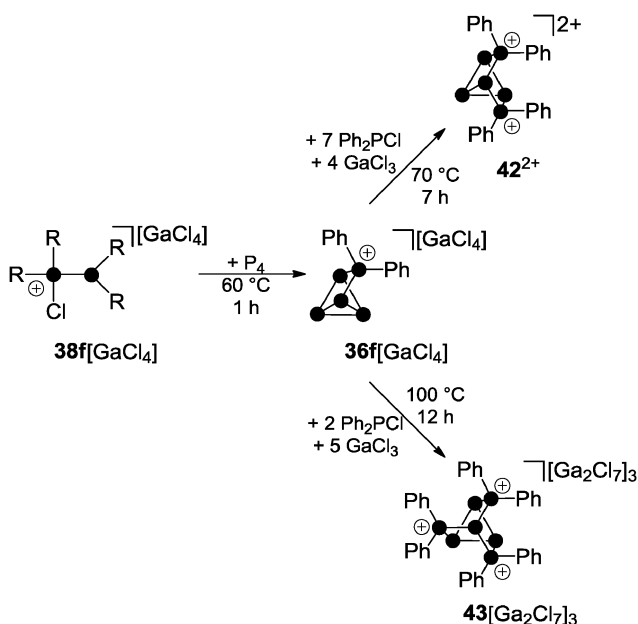
Scheme 12 Stepwise insertion of Ph_2P^+ -phosphonium ions into P–P bonds of P_4 yielding Ph_4P_6^{2+} -cage cation 42 2+ and Ph_6P_7^{3+} -cage compound 43 [Ga_2Cl_7]_3 .
