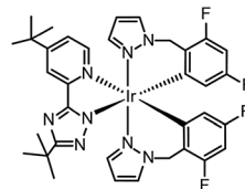
\text{Ir}(\text{dfb-pz})_2(\text{bbptz}) 53
