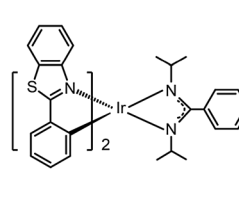
(bt) 2 Ir(dipba) 218
