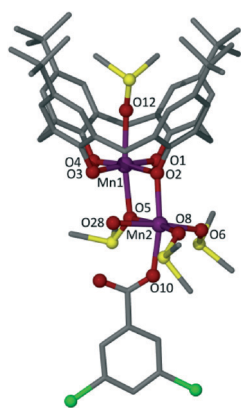
Fig. 2 Partially labelled structure of 1 showing the 3,5-dichlorobenzoate appended to the Mn III Mn II cluster core, ligation of DMSO in the TBC[4] cavity and both bridging and terminal ligated solvent. Colour code: C – grey, O – red, S – yellow, Mn – purple, Cl – green. H atoms omitted for clarity.
