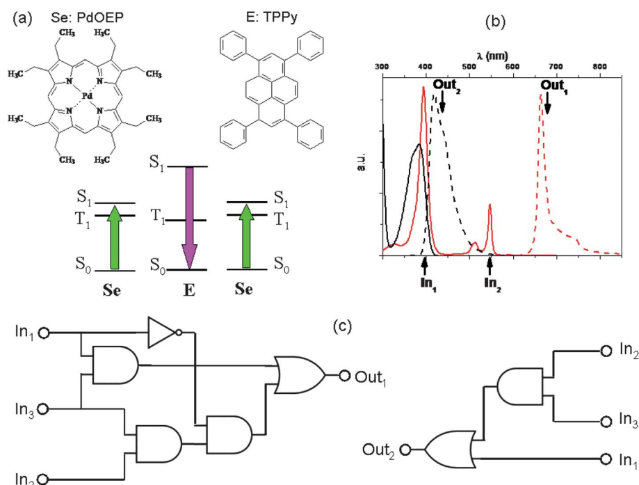
Fig. 7 A TTA up-conversion process involving PdOEP as sensitizer (Se) and TPPy as emitter (E), whose molecular structures are in (a) along with a scheme of their relative energy levels. The pair PdOEP–TPPy convert green light into violet light. In (b) the continuous traces represent the absorption spectra (in black that of TPPy and in red that of PdOEP), whereas the dashed traces represent the emission spectra (black for TPPy and red for PdOEP). (c) If we choose \lambda_{\text{exc}} = 400 \text{ nm} , \lambda_{\text{exc}} = 546 \text{ nm} and \text{N}_2 as the first ( \text{In}_1 ), second ( \text{In}_2 ) and third ( \text{In}_3 ) inputs, respectively, complicated binary logic circuits can be implemented with the phosphorescence of PdOEP ( \text{Out}_1 ) and the fluorescence signal of TPPy ( \text{Out}_2 ) as outputs.
