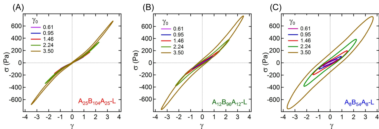
Fig. 3 Lissajous plots obtained from amplitude sweep experiments displaying the shear stress ( \sigma ) vs. intracycle strain ( \gamma ) for (A) A_{25}B_{104}A_{25} -L, (B) A_{12}B_{96}A_{12} -L, and (C) A_8B_{54}A_8 -L for \gamma_0 \approx 0.61, 0.95, 1.46, 2.24, and 3.50 . The experiments were performed using oscillatory frequency ( \omega ) of 1 rad/s.
