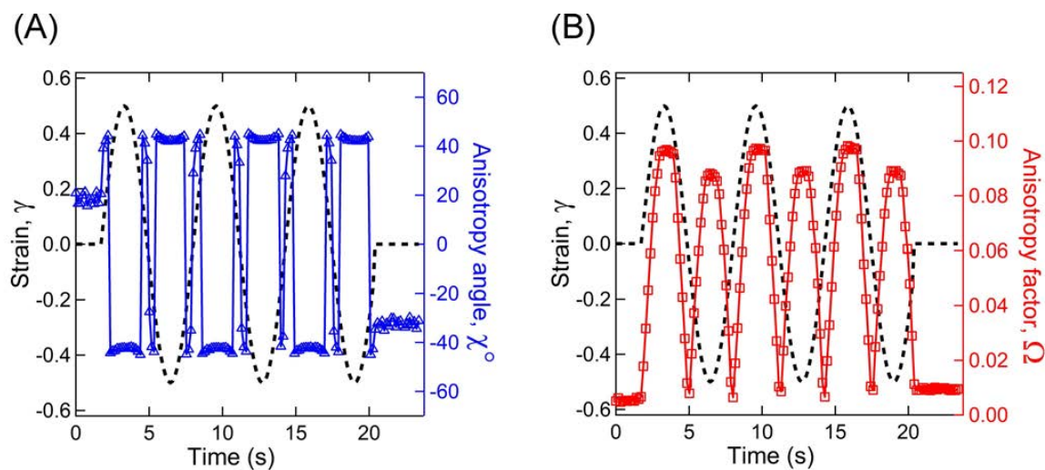
Fig. 11 Estimated anisotropic factor and angle for A_{12}B_{96}A_{12} -H. (A) Strain ( \gamma ) on left-y-axis and anisotropy angle ( \chi ) on right-y-axis as a function of time. (B) \gamma on left-y-axis and anisotropy factor ( \Omega ) on right-y-axis as a function of time. RheoSAXS experiments were performed with an oscillatory \gamma_0=0.5 and \omega=1 rad/s.
