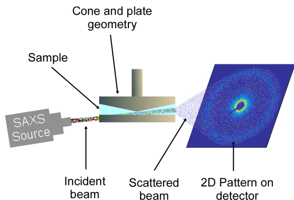
Fig. 1 Schematic of RheoSAXS setup where X-ray beam passed through a hole at the bottom plate at 5^\circ angle and then through the sample capturing the scattering data in 1-2 plane.
