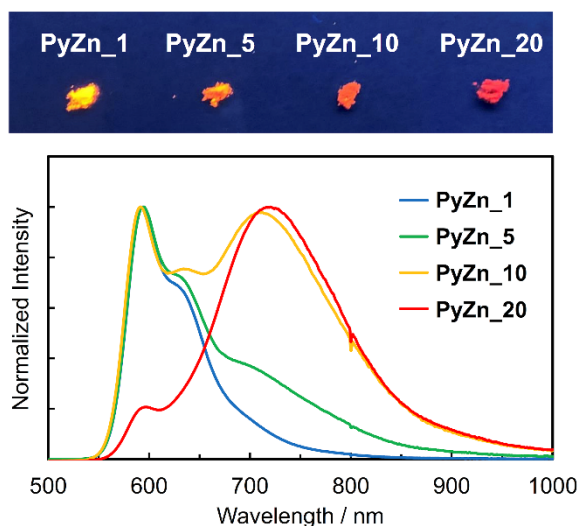
Fig. 3 Normalized emission spectra (lower, \lambda_{\text{ex}} = 370 \text{ nm} ) and photograph (upper, \lambda_{\text{ex}} = 365 \text{ nm} ) of \text{PyZn}_R .
