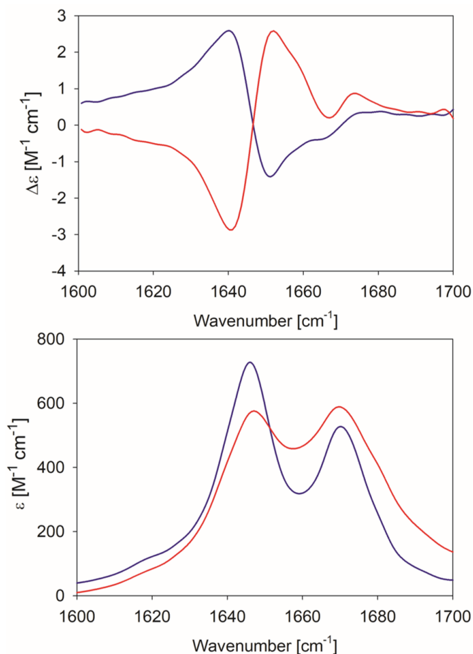
Fig. 1 Amide I' region of the VCD (upper panel) and IR (lower panel) spectra of the GAG gel phase at 10°C (blue) and 23°C (red). The two VCD spectra and the IR spectrum of the 10°C gel phase were already reported by Farrell et al. 30
