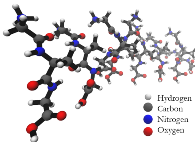
Fig. 5 Structure of the geometry optimized octamer of GAG with parallel oriented peptides.
