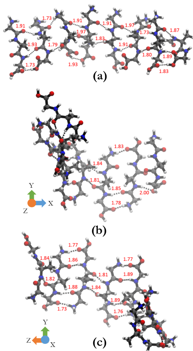
Fig. 8 (a) Hydrogen bonding between peptide groups in the octamer with parallel orientation. (b) and (c) show the hydrogen bonding in the antiparallel orientation. (b) and (c) are the same structure rotated by 90° around the y-axis to aid the visualization of all the bonds in the structure. Hydrogen bonds are shown in black dotted lines and the hydrogen bond lengths are shown in red.
