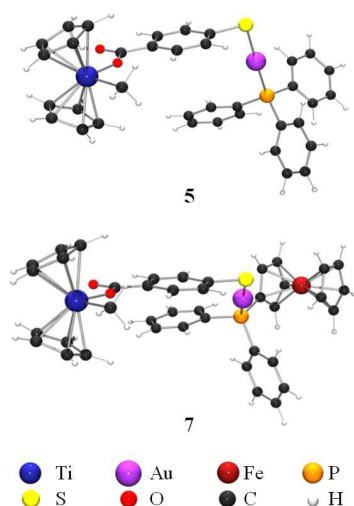
Figure 3. Optimized structures for heterometallic complexes 5 and 7 .
