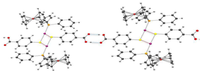
Figure 2. ORTEP view of the polymeric structure of 6 showing hydrogen bonds (blue dotted line) and the Au-S weak interactions (red-brown dotted line). Applied colour code as in Figure 1.
