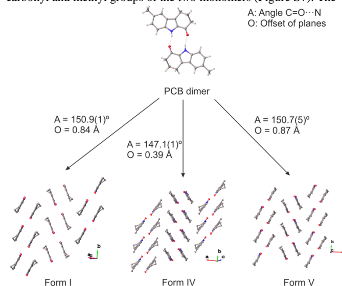
Figure 3 Crystal packing of the three polymorphs of PCB as determined by single-crystal X-ray diffraction.
