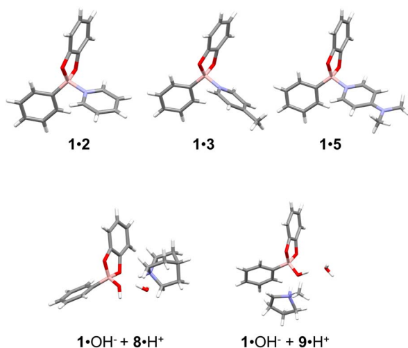
Fig. 2 Perspective view of the X-ray molecular structures. Top row: adducts 1 \cdot 2 , 1 \cdot 3 , 70 and 1 \cdot 5 . Bottom row: co-crystals 1 \cdot OH^- + 8 \cdot H^+ and 1 \cdot OH^- + 9 \cdot H^+ Colour code: B, pink; N, blue; O, red; C, grey; H, white.
