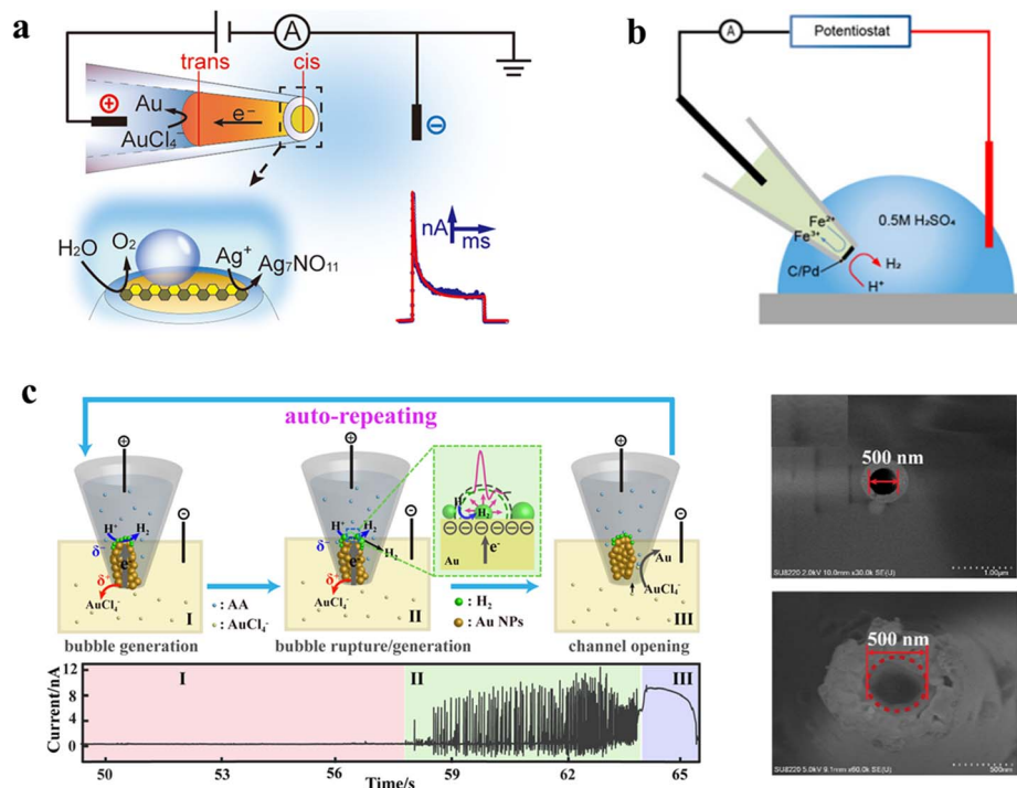
Fig. 3 Single-entity electrocatalytic analysis using WNEs. (a) A closed-type WNE for in situ and real-time monitoring of the electrocatalytic performance of Ag 7 -NO 11 in the oxygen evolution reaction. Reproduced with permission. 56 Copyright 2022, American Chemical Society. (b) The WNE loaded with a C/Pd catalyst for monitoring the HER. Reproduced with permission. 57 Copyright 2023, Royal Society of Chemistry. (c) Left: monitoring the auto-repeating bipolar reactions and HER on a AuNP-confined WNE: (I) bubble generation, (II) bubble rupture/generation, and (III) channel opening (top). The current–time trace of the first cycle for the AuNP-confined WNE at 1.2 V: (I) the low baseline region, (II) the current pulse region, and (III) the baseline increase region (bottom). Right: SEM image of the orifice with a 500 nm diameter before (top) and after (bottom) blocking the AuNPs. Reproduced with permission. 60 Copyright 2023, American Chemical Society.
