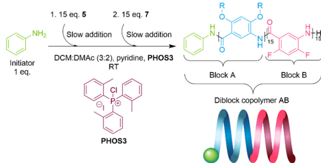
Scheme 2 Top: Synthetic paths for monomers 5 and 7 . (a) \text{K}_2\text{CO}_3 , DMF, 15-bromo-2,5,8,11-tetraoxapentadecane 2 , 51%. (b) \text{H}_2/\text{Pd}/\text{C} , MeOH, EtOAc, quant. (c) KOH, EtOH, 60%. (d) \text{H}_2/\text{Pd}/\text{C} , MeOH, EtOAc, quant. Bottom: Polymerization conditions of diblock copolymer AB.
