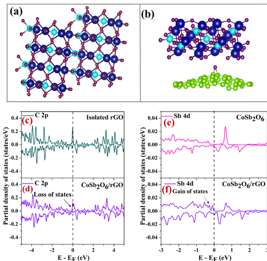
Fig. 8 (a) and (b) Optimised structures of the (110) surface of \text{CoSb}_2\text{O}_6 and \text{CoSb}_2\text{O}_6/\text{rGO} , respectively. The blue, cyan, purple, and green spheres represent Sb, Co, O, and C atoms. (c) and (d) Partial density of states plots for the C 2p orbital of isolated rGO and the \text{CoSb}_2\text{O}_6/\text{rGO} composite, respectively. (e) and (f) Partial density of states plots for the Sb 4d orbital of the (110) surface of \text{CoSb}_2\text{O}_6 and the \text{CoSb}_2\text{O}_6/\text{rGO} composite, respectively. The dotted line drawn vertically at 0 eV on the x-axis represents the Fermi level.
