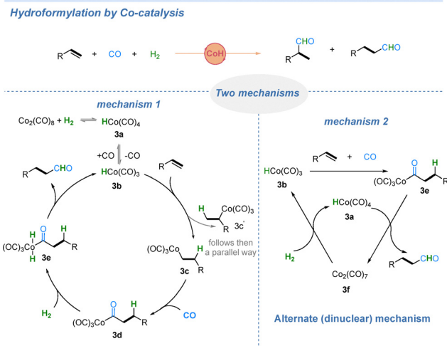
Scheme 3 Cobalt-catalyzed hydroformylation of alkenes.
