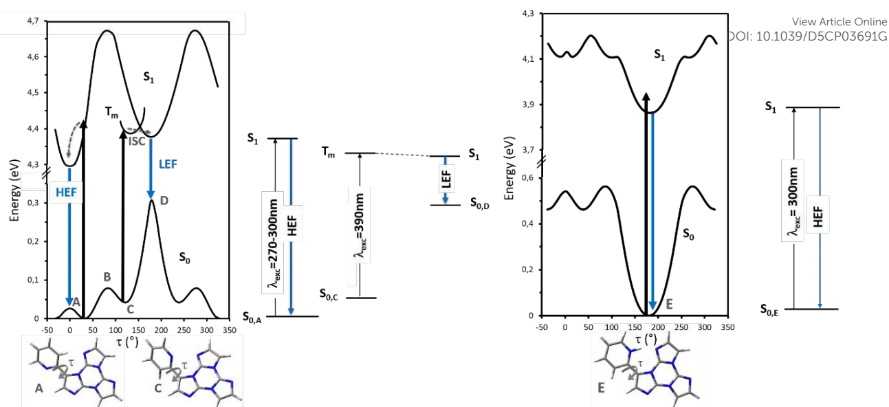
Fig. 2 Scans of the relaxed potential energy surfaces of S_1 and S_0 and simplified Jablonski diagrams for fluorescent emissions of TT-2Py (left) and TT-2PyH + (right) along the N_{py}-C_{py}-C_{TT}-C_{TT} torsion angle, \tau , at the (TD)- \omega B97X/6-311++G(d,p) level of theory. T_m represents a generic triplet level, A, C and E denote minima on S_0 of TT-2Py and TT-2PyH + and B is the barrier between the two minima on S_0 of TT-2Py . Energies are relative to the S_0 state equilibrium geometry.
