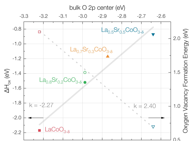
Figure 4. Correlation of experimental oxidation enthalpies \Delta H_{\text{ox}} of \text{La}_{1-x}\text{Sr}_x\text{CoO}_{3-\delta} with x = 0-0.5 52 (left y-axis) and V_{\text{O}}^{\bullet} formation energies 40 (right y-axis) plotted against the calculated bulk O 2p band centers of the respective composition (obtained from interpolation of literature results 53 )
