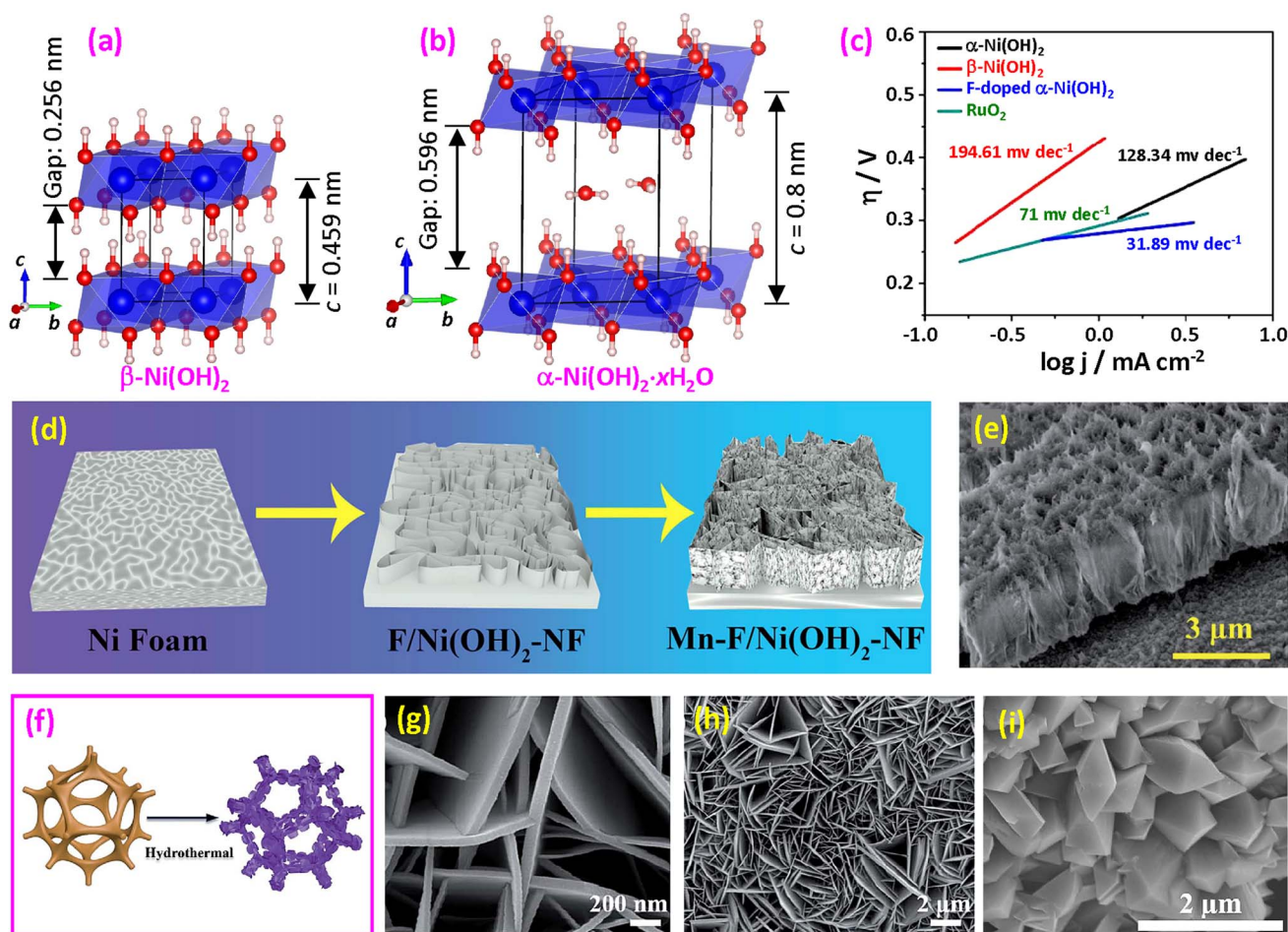
Fig. 10 (a) Structural model of \beta -Ni(OH) 2 ; (b) structural model of \alpha -Ni(OH) 2 . (c) Tafel slope of OER catalysts. Reproduced from ref. 161 with permission from the Royal Society of Chemistry, copyright 2019. (d) Synthesis of Mn and F doped Ni(OH) 2 on NF and (e) SEM side view of Mn-F/Ni(OH) 2 -NF. Reproduced from ref. 162 with open access. (f) Synthesis of Co x Fe 1-x (OH)F via a one-step hydrothermal procedure; (g and h) SEM images. Reproduced from ref. 163 with permission from the Royal Society of Chemistry, copyright 2022. (i) SEM image of Co(OH)F. Reproduced from ref. 164 with permission from Elsevier, copyright 2022.
