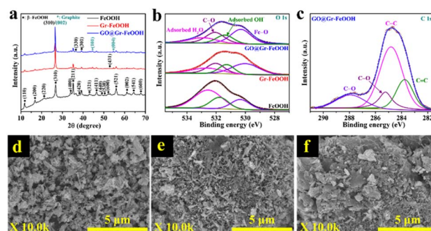
Fig. 1 (a) XRD patterns, (b) XPS spectra of O 1s for FeOOH, Gr-FeOOH and GO@Gr-FeOOH samples, (c) XPS spectra of C 1s for the GO@Gr-FeOOH sample; HR FE-SEM top view images of (d) FeOOH, (e) Gr-FeOOH and (f) GO@Gr-FeOOH samples.
