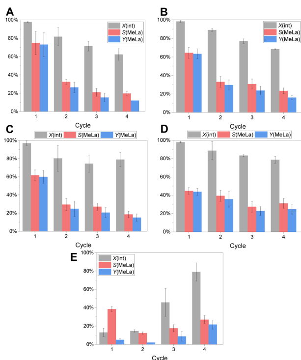
Fig. 3 Conversion of PLA ( X(\text{int}) , black), selectivity towards methyl lactate ( S(\text{MeLa}) , red), and yield of methyl lactate ( Y(\text{MeLa}) , blue) for the repeatedly performed methanolysis of PLA under aerobic conditions recycling the catalyst after each reaction cycle. Used catalysts: B-TMGtegma+ 5 mol% (A), SB-TMGtegma+ 5 mol% (B), B-TMGtegma+ 15 mol% (C), SB-TMGtegma+ 15 mol% (D), and as reference experiment TMGtegma+ (E). Average values of a threefold determination with standard deviation are displayed.
