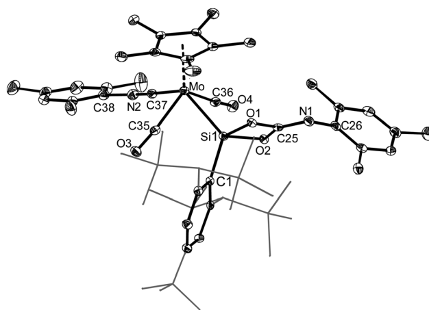
Fig. 6 DIAMOND plot of the molecular structure of 2-Mo . Thermal ellipsoids are set at 30% probability, hydrogen atoms were omitted and the substituents of the Tbb group are presented as wireframe for the sake of clarity. Selected bond lengths (pm) and bond angles (°): for 2-Mo (bond lengths and bond angles of 2-W are given in square brackets): Mo–Si1 253.01(7) [253.5(1)], Mo–C35 198.8(3) [198.8(5)], Mo–C36 197.8(3) [197.2(5)], Mo–C37 204.2(3) [204.2(5)], Si1–O1 174.8(2) [175.4(3)], Si1–O2 176.0(2) [175.9(3)], Si1–C1 188.8(2) [187.9(4)], O1–C25 135.9(3) [135.6(5)], O2–C25 136.0(3) [136.6(5)], N1–C25 125.9(3) [125.7(5)], Si1–Mo–C35 74.11(7) [75.2(1)], Si1–Mo–C37 127.7(1) [128.4(1)], C35–Mo–C36 110.3(1) [111.6(2)], O1–Si1–O2 75.69(8) [75.7(1)], O1–C25–O2 104.6(2) [104.8(3)], Si1–O1–C25 90.1(1) [90.0(2)], Si1–O2–C25 89.5(1) [89.5(2)].
