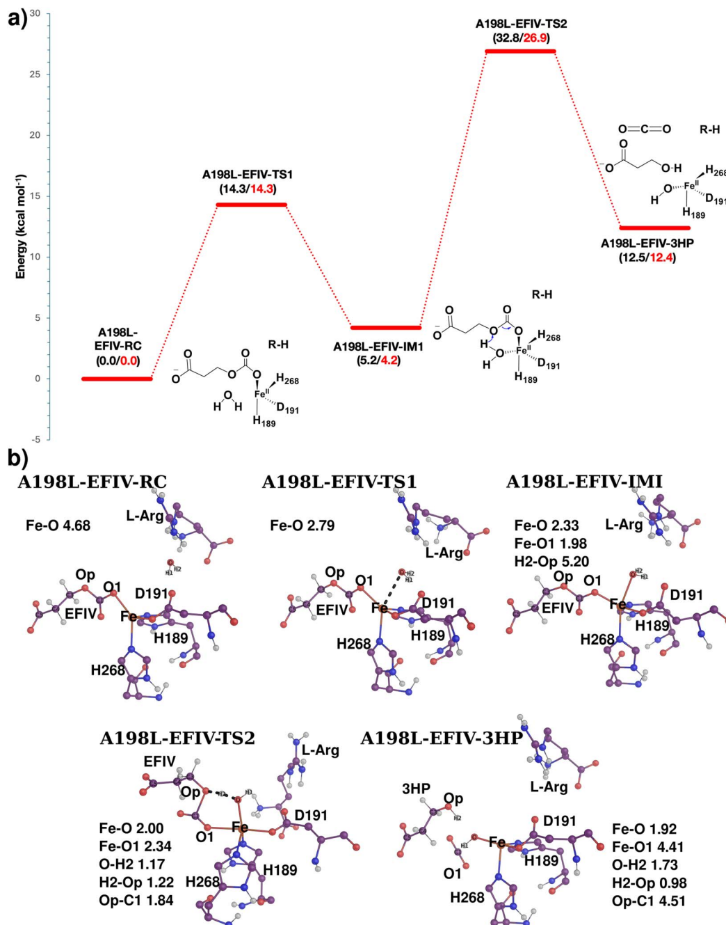
Fig. 10 (a) Reaction profile of the 3HP formation mechanism in A198L EFE. Relative energies are given in \text{kcal mol}^{-1} at QM(B2)/MM (black) and QM(B3)/MM (red) levels. The profile was plotted at QM(B3)/MM levels. (b) The optimized geometries of the intermediates and transition states obtained during the QM/MM simulations.
