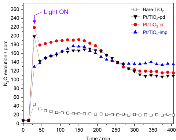
Fig. 3 \text{N}_2\text{O} evolutions over different photocatalysts. Photocatalytic tests were carried out at an SV of 3500 \text{ h}^{-1} .
