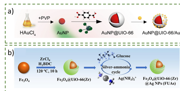
Fig. 9 Schematic diagram of the fabrication of (a) AuNP@UiO-66/Au nanoparticles 49 and (b) Fe 3 O 4 @UiO-66(Zr)@AgNPs. 50 Reprinted with permission from ref. 49. Copyright 2023 Royal Society of Chemistry. Reprinted with permission from ref. 50. Copyright 2023, with permission from Elsevier.
