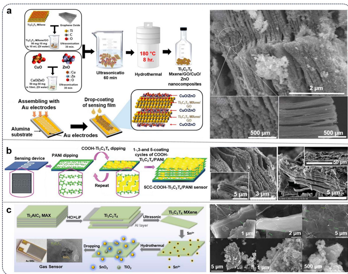
Fig. 2 (a) Synthesis schematic diagram of \text{Ti}_3\text{C}_2\text{T}_x MXene/GO/CuO/ZnO nanocomposites. 90 (b) Schematic of sensor fabrication process using dip-method and coating cycles of \text{COOH-Ti}_3\text{C}_2\text{T}_x/\text{PANI} . 91 (c) Illustration of preparation process of \text{Ti}_3\text{C}_2\text{T}_x\text{-SnO}_2 nanocomposite. The right side includes SEM images of the as-prepared MXene composites. 92
