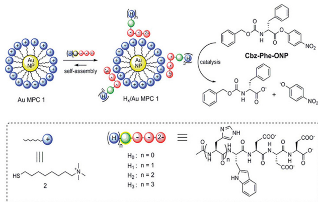
Fig. 13 Self-assembly of peptides H0–H3 on the surface of an Au MPC, followed by the formation of H_x/Au MPC complexes that ( x = 1–3 ) that can catalyze the transesterification of the substrate Cbz-Phe-ONP. Adapted with permission from ref. 172. Copyright 2012 American Chemical Society.
